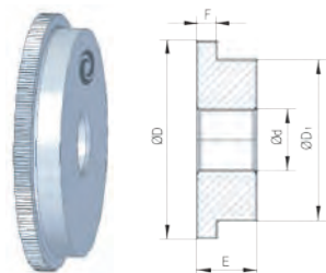
Moleta escalonada (una cara) Stepped knurl (one side)
